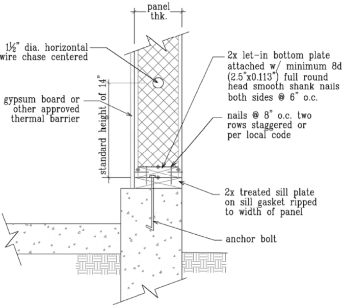
FIGURE 3—TYPICAL WALL PANEL ON FOUNDATION
