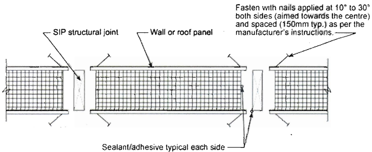
Figure 1. “Insulspan SIP System” wall panels with lumber studs at 1.2 m o.c. Note that lumber studs, top and bottom plates are installed in the field following a specific nailing schedule. See manufacturer’s installation details.
